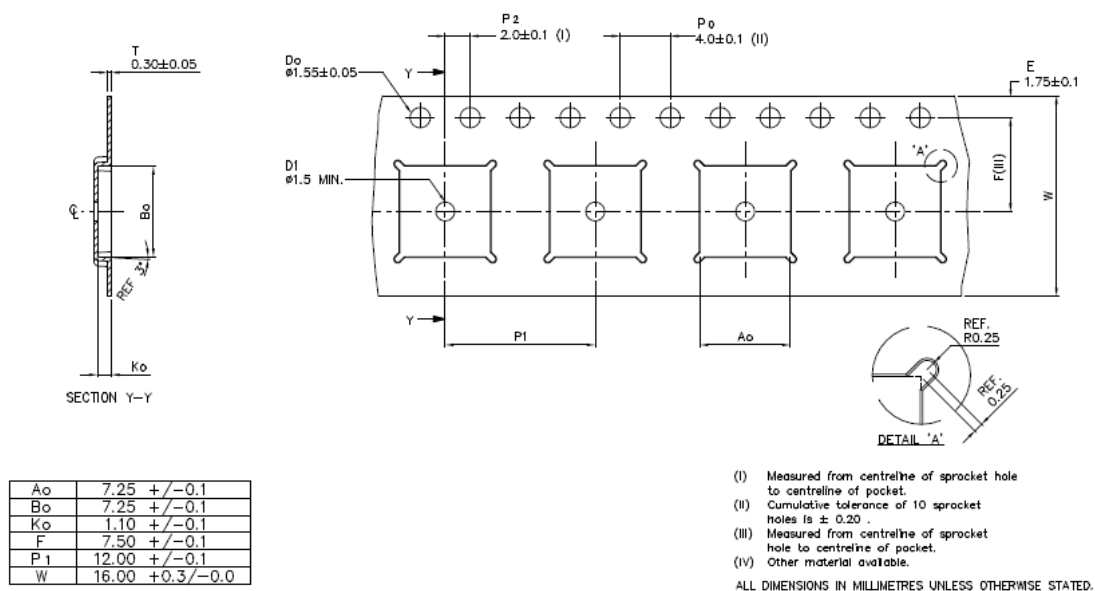
Figure 24. Detailed Tape and Reel Dimensions
