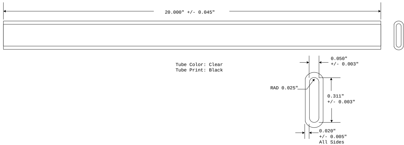
Figure 25. Tube dimension (in inches)
